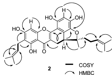
Figure 3. COSY and key HMBC correlations of 2 .
