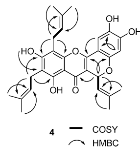
Figure 6. COSY and key HMBC correlations of 4 .
