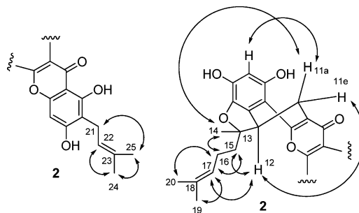
Figure 4. Selected NOESY correlations of 2 .
