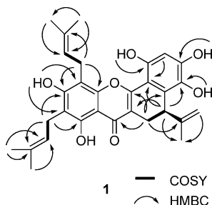
Figure 1. COSY and key HMBC correlations of 1 .
