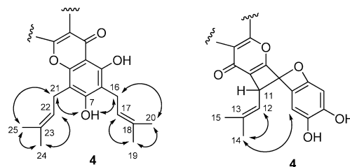
Figure 7. Selected NOESY correlations of 4 .
